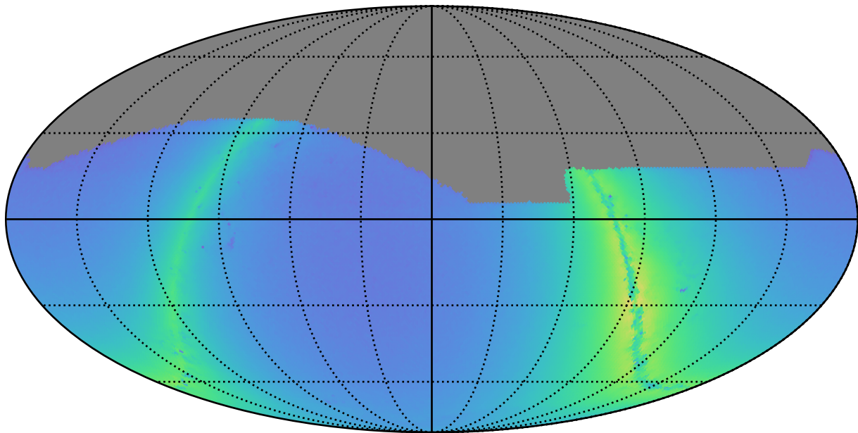
reweight_bulge_v3.3_10yrs i: Nstars_no_crowding
