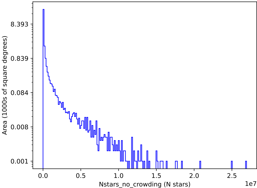
reweight_bulge_v3.3_10yrs i: Nstars_no_crowding
