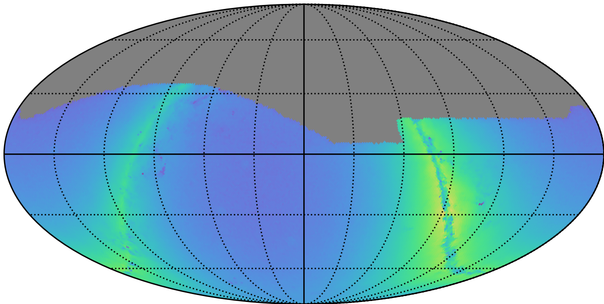
reweight_bulge_v3.3_10yrs g: Nstars_no_crowding
