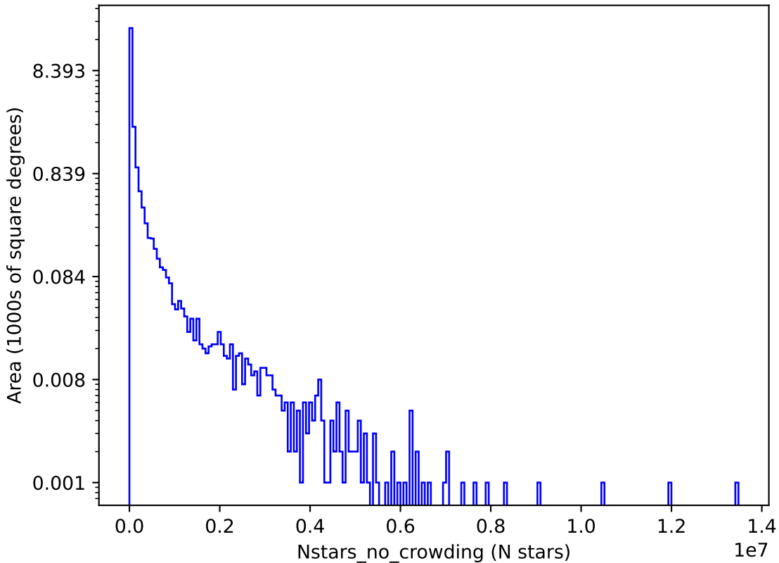
reweight_bulge_v3.3_10yrs g: Nstars_no_crowding
