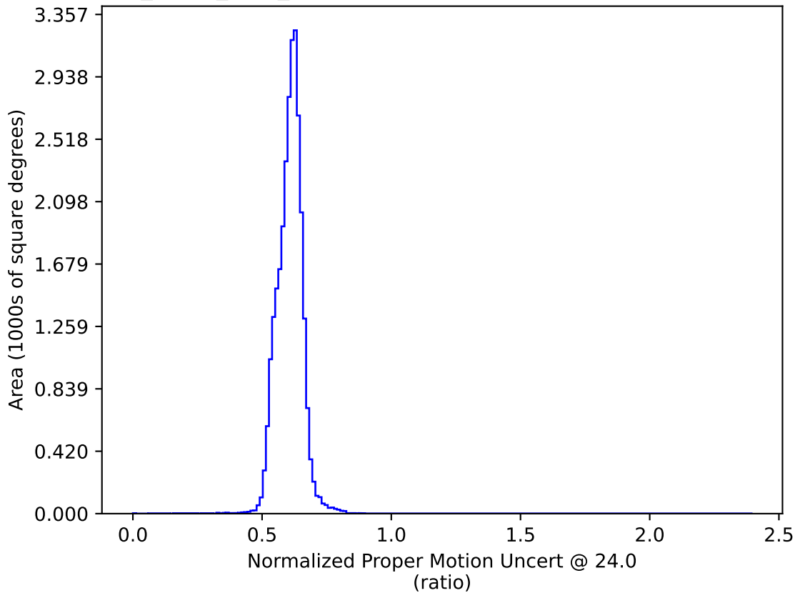
reweight_bulge_v3.3_10yrs : Normalized Proper Motion Uncert @ 24.0
