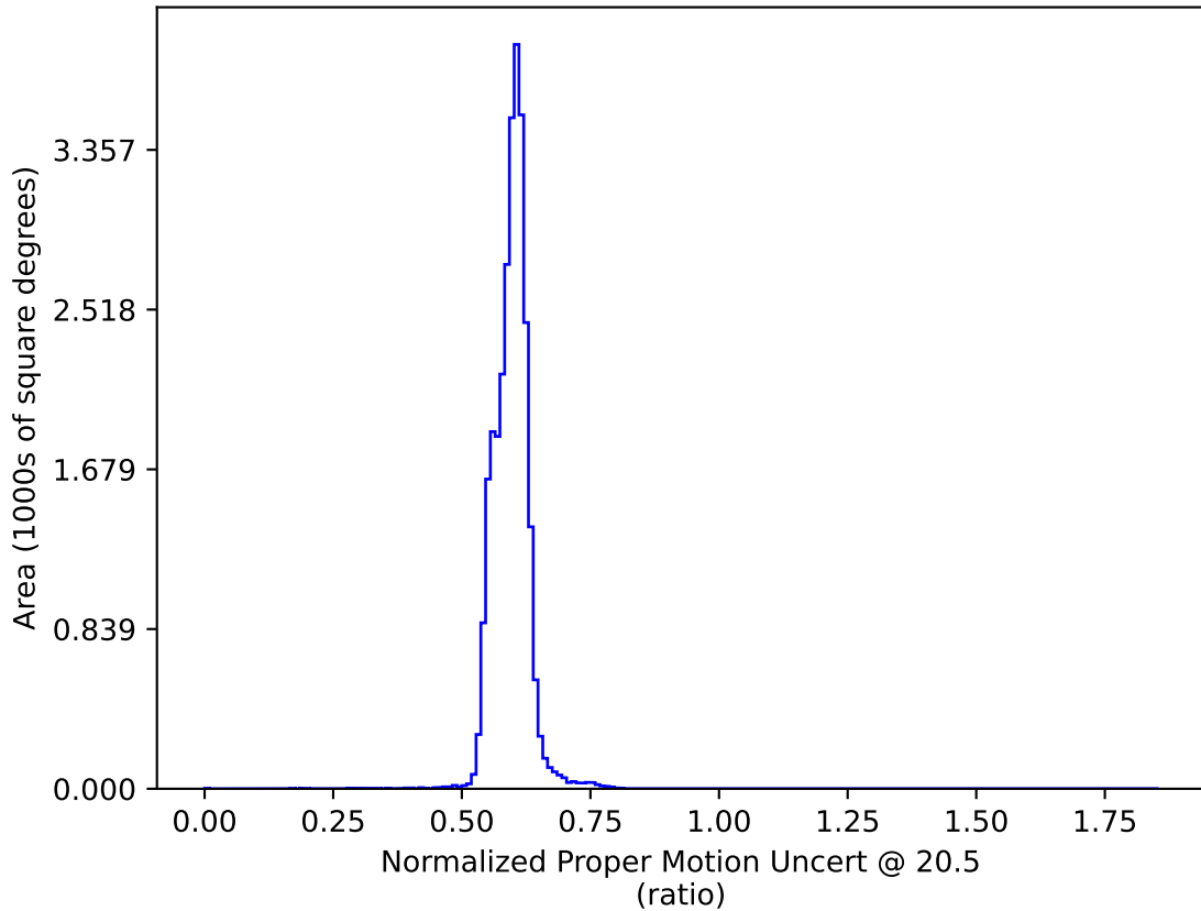
reweight_bulge_v3.3_10yrs : Normalized Proper Motion Uncert @ 20.5
