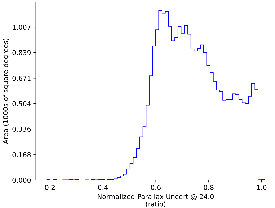
reweight_bulge_v3.3_10yrs : Normalized Parallax Uncert @ 24.0
