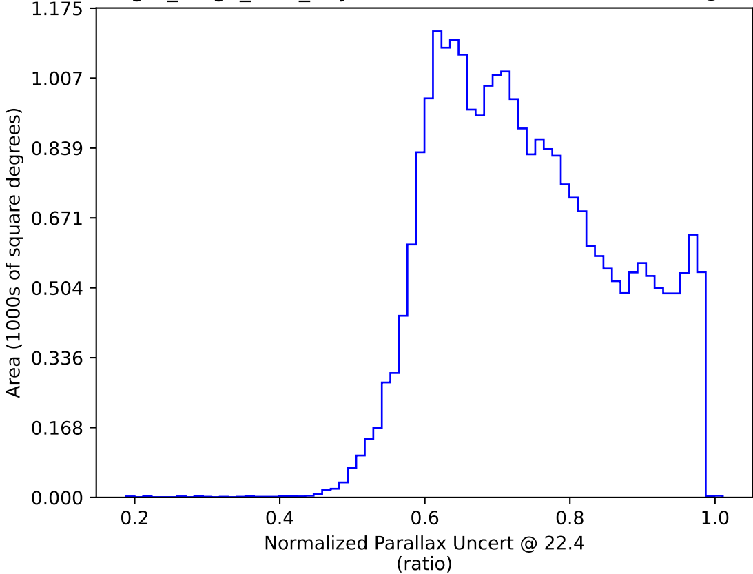
reweight_bulge_v3.3_10yrs : Normalized Parallax Uncert @ 22.4
