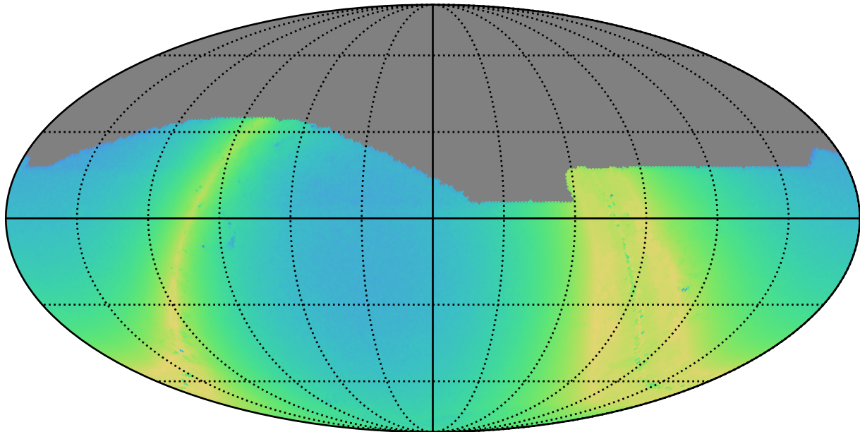
reweight_bulge_v3.3_10yrs z: N stars to Precision 0.20
