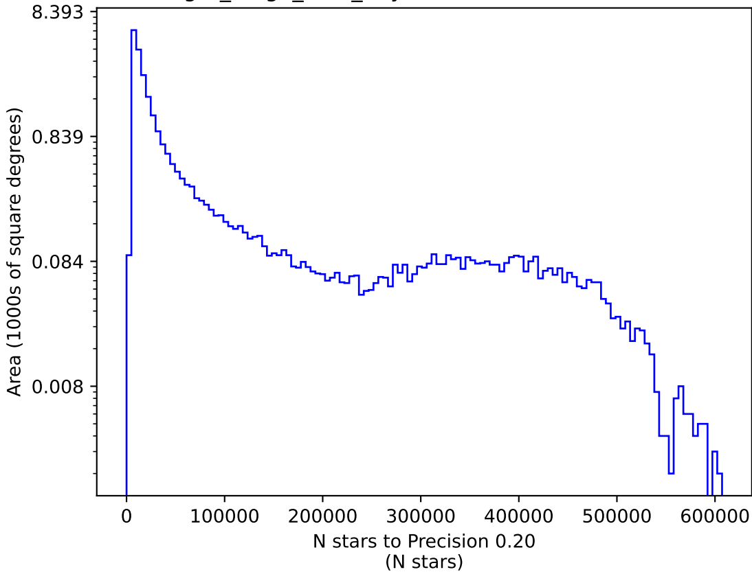
reweight_bulge_v3.3_10yrs z: N stars to Precision 0.20
