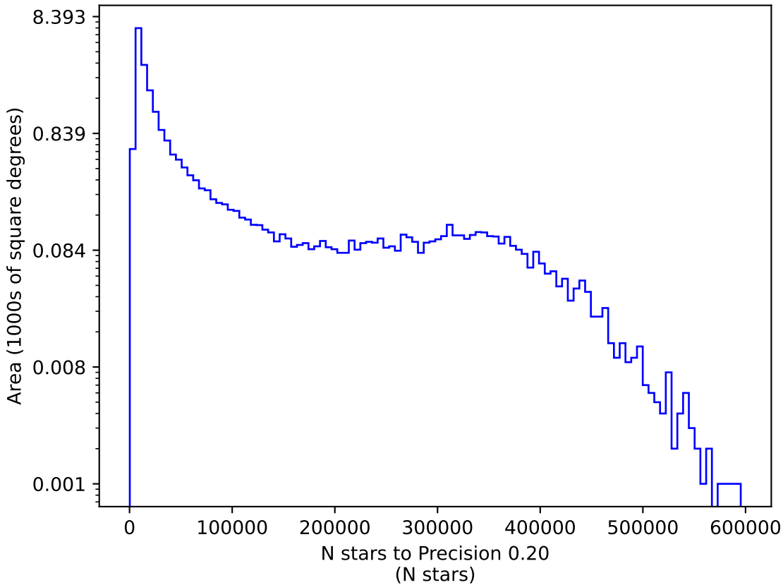
reweight_bulge_v3.3_10yrs y: N stars to Precision 0.20
