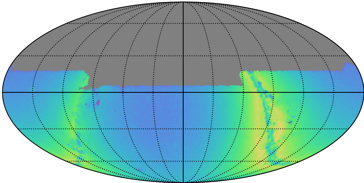
reweight_bulge_v3.3_10yrs u: N stars to Precision 0.20
