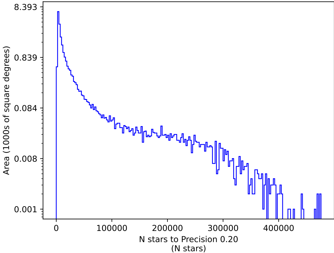
reweight_bulge_v3.3_10yrs u: N stars to Precision 0.20
