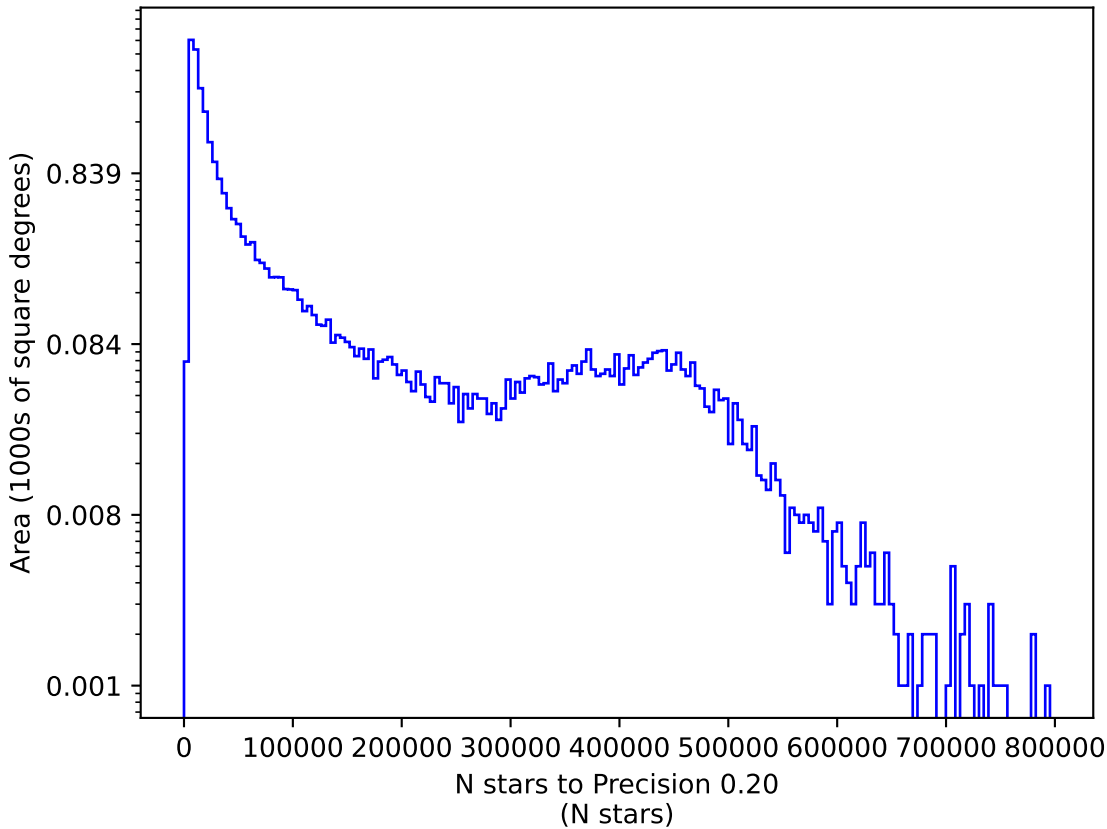
reweight_bulge_v3.3_10yrs r: N stars to Precision 0.20
