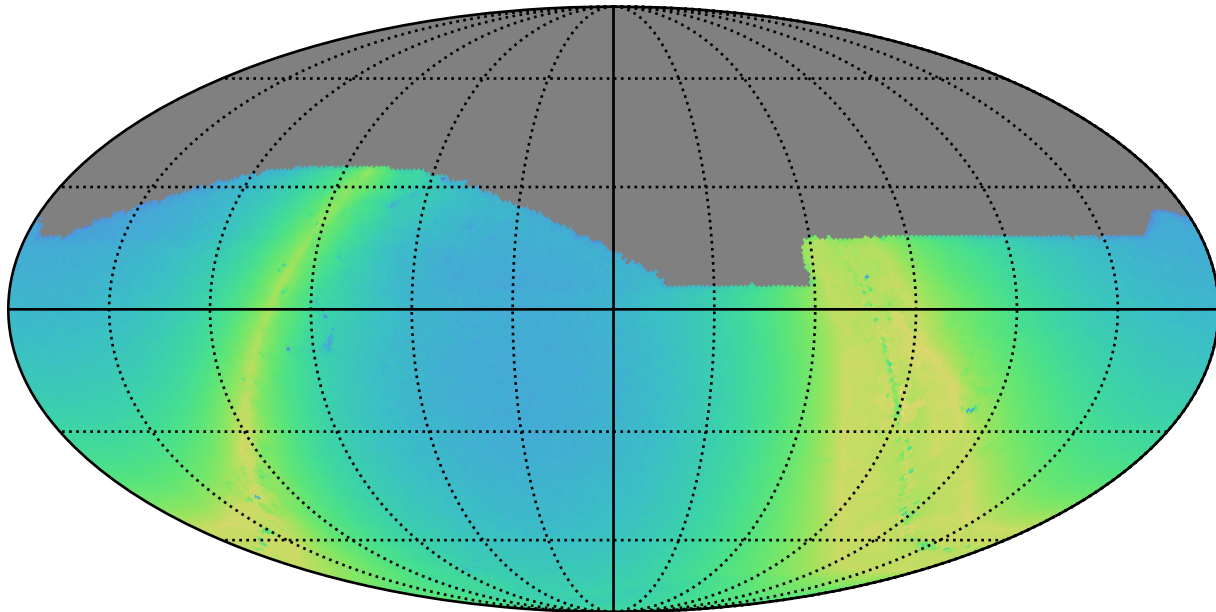
reweight_bulge_v3.3_10yrs i: N stars to Precision 0.20
