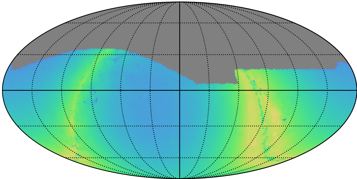
reweight_bulge_v3.3_10yrs g: N stars to Precision 0.20
