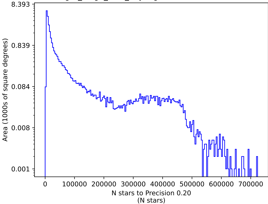
reweight_bulge_v3.3_10yrs g: N stars to Precision 0.20
