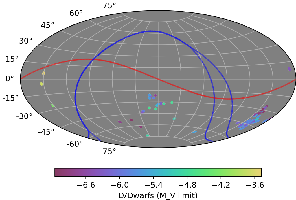
reweight_bulge_v3.3_10yrs gi: LVDwarfs
