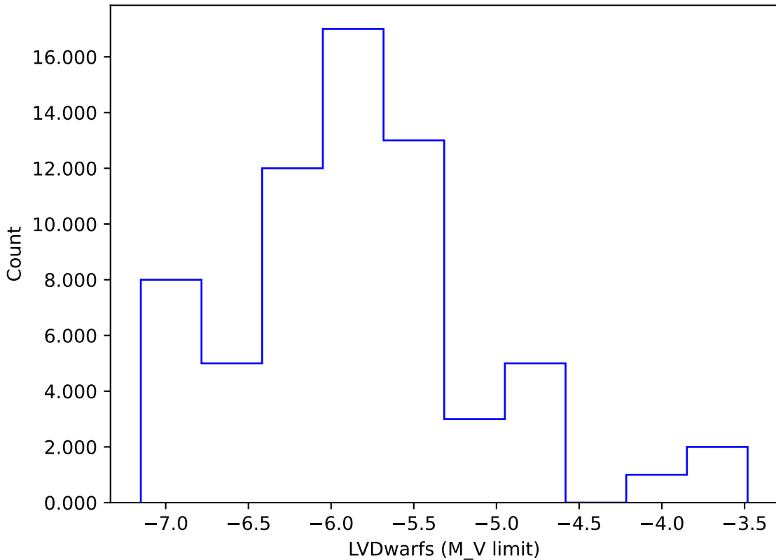
reweight_bulge_v3.3_10yrs gi: LVDwarfs
