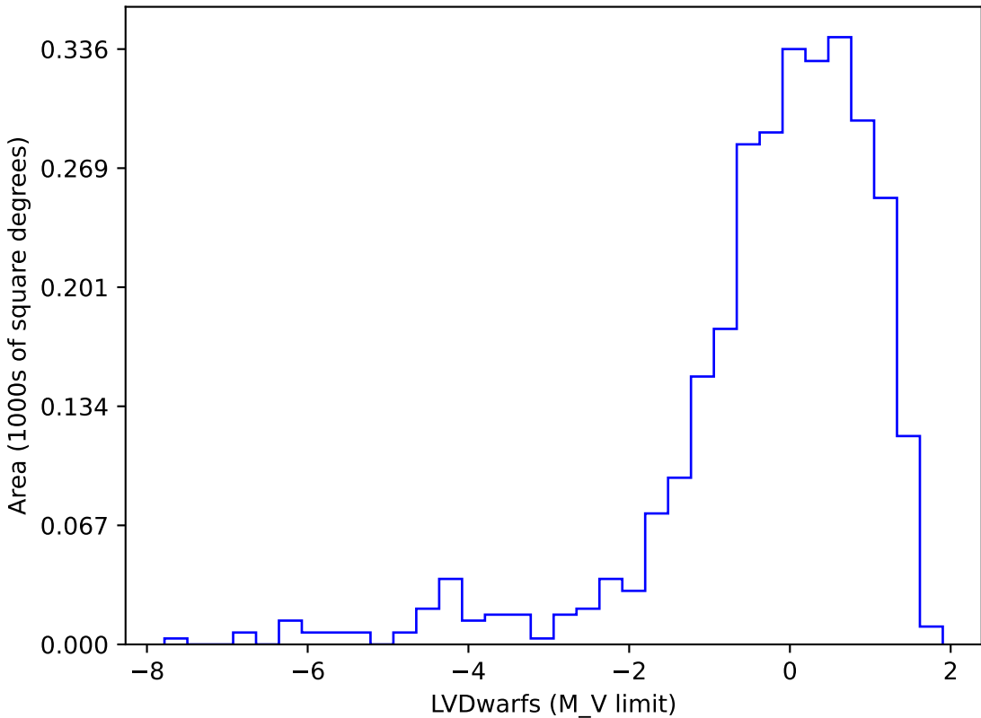
reweight_bulge_v3.3_10yrs gi SCP: LVDwarfs
