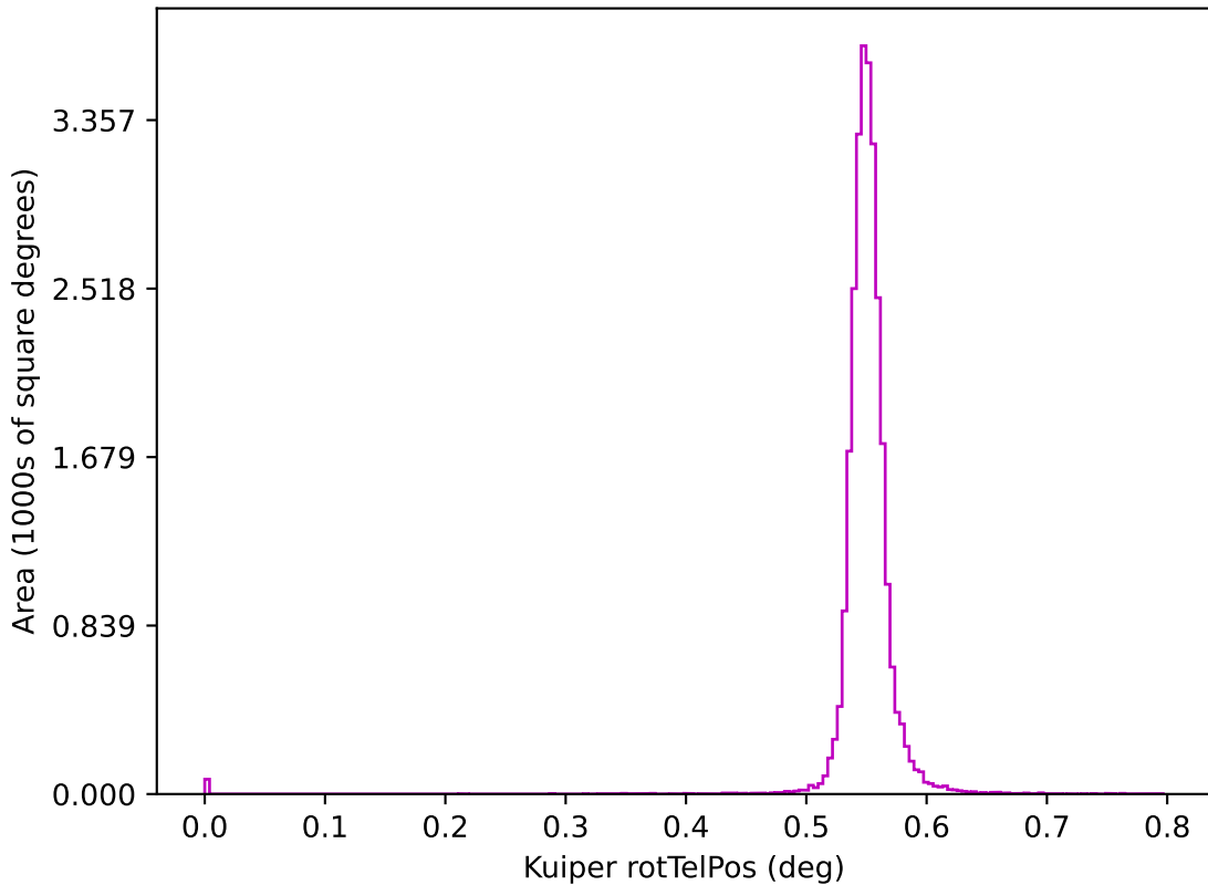
reweight_bulge_v3.3_10yrs z: Kuiper rotTelPos
