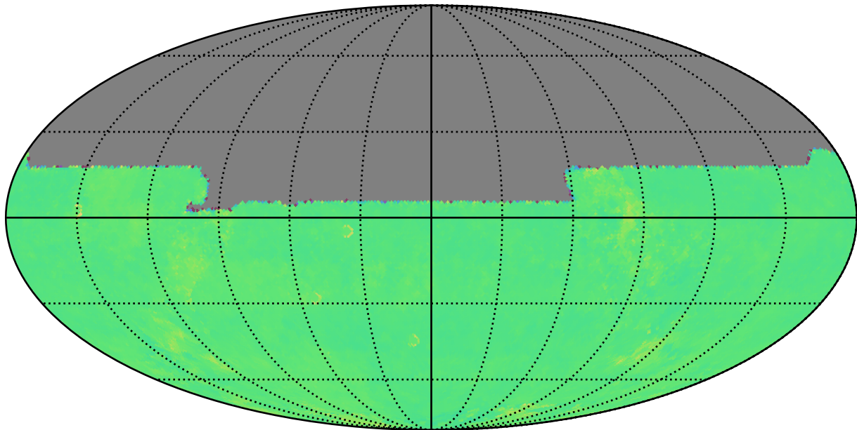
reweight_bulge_v3.3_10yrs y: Kuiper rotTelPos
