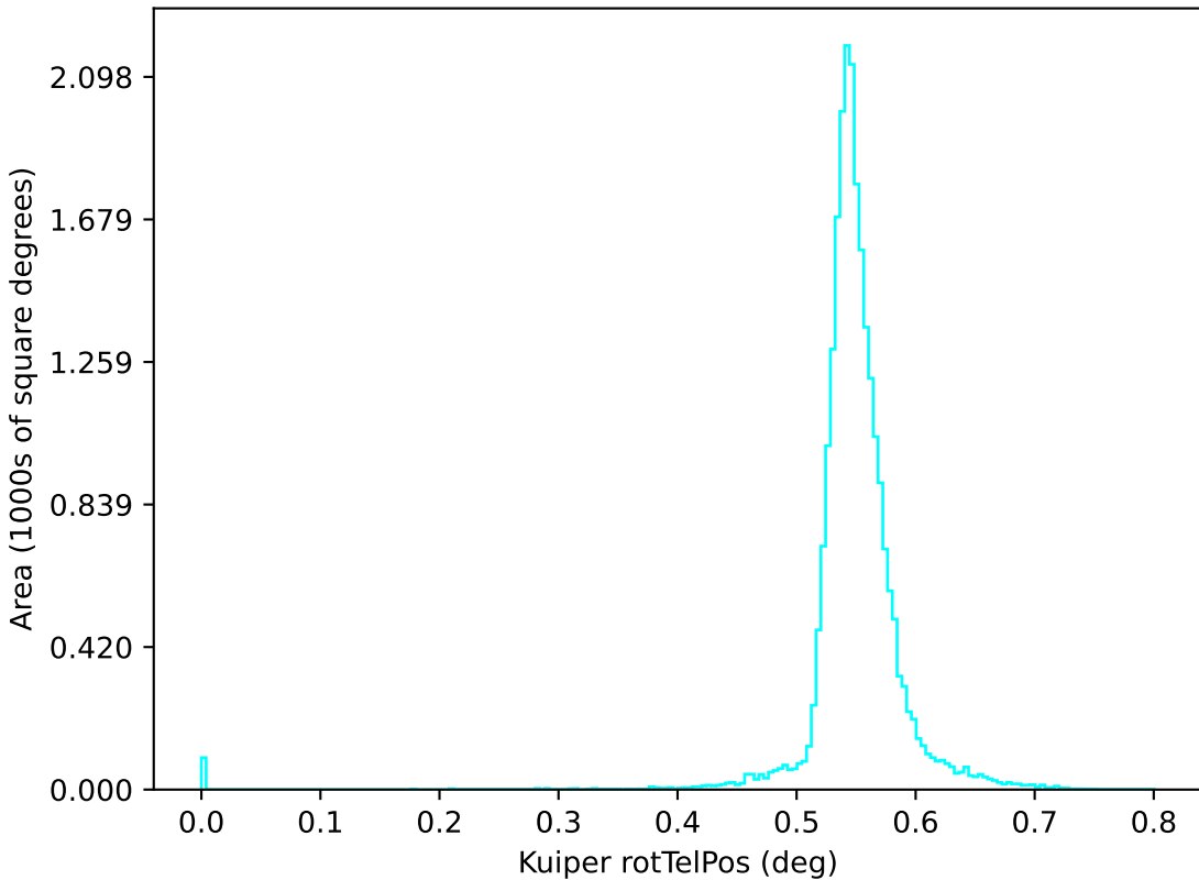
reweight_bulge_v3.3_10yrs u: Kuiper rotTelPos
