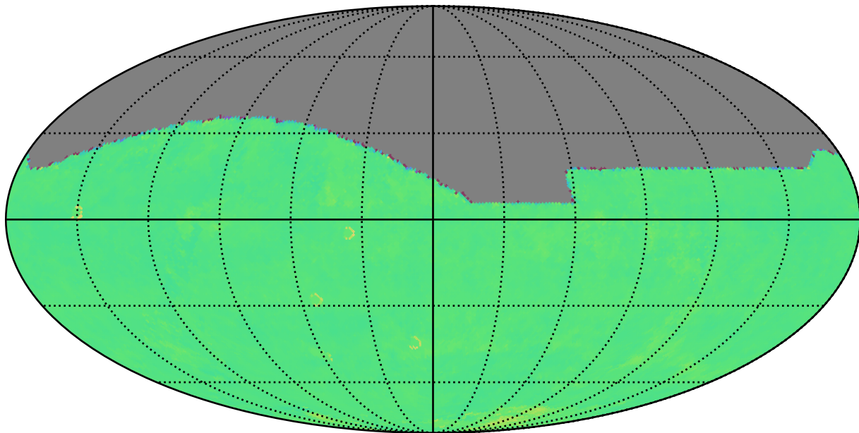
reweight_bulge_v3.3_10yrs r: Kuiper rotTelPos
