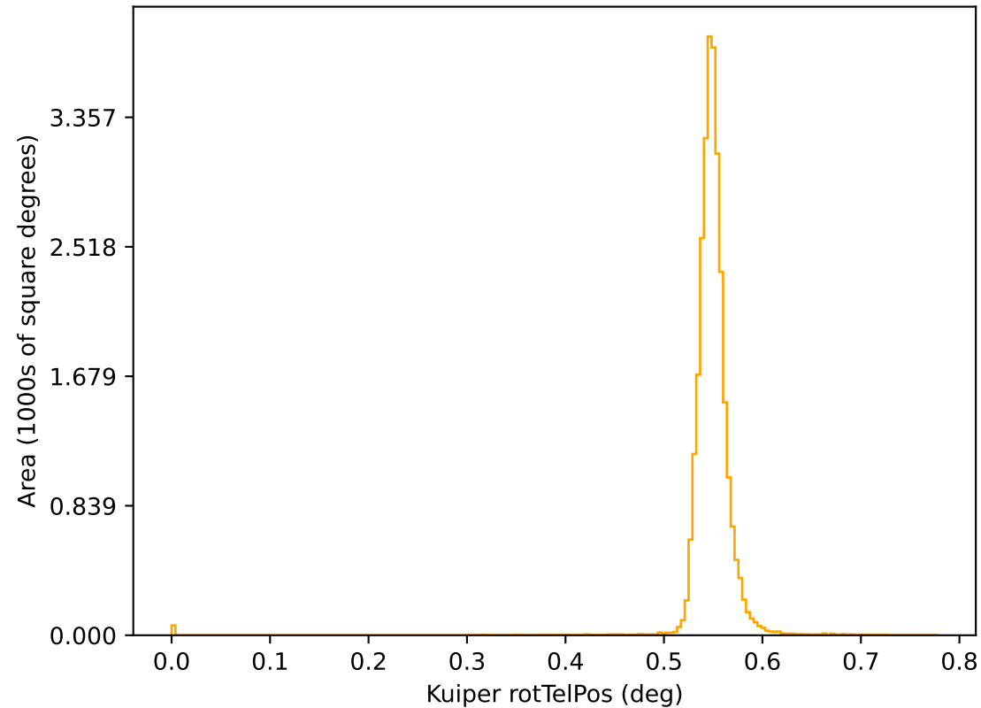
reweight_bulge_v3.3_10yrs r: Kuiper rotTelPos
