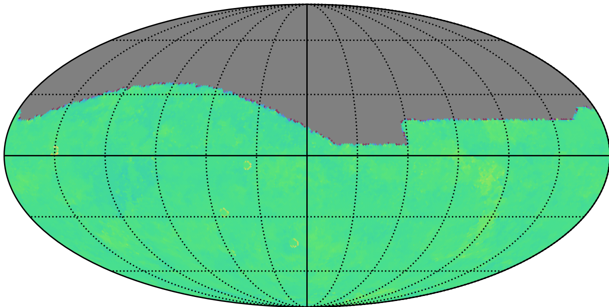
reweight_bulge_v3.3_10yrs g: Kuiper rotTelPos
