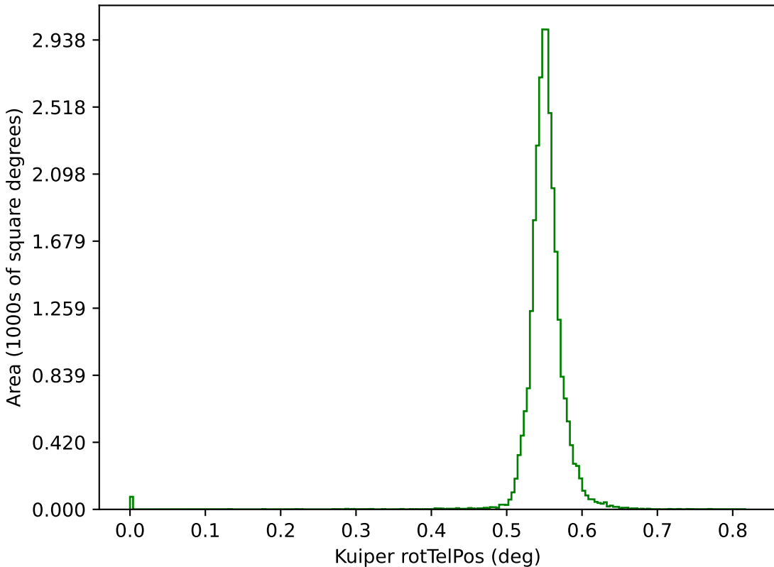
reweight_bulge_v3.3_10yrs g: Kuiper rotTelPos
