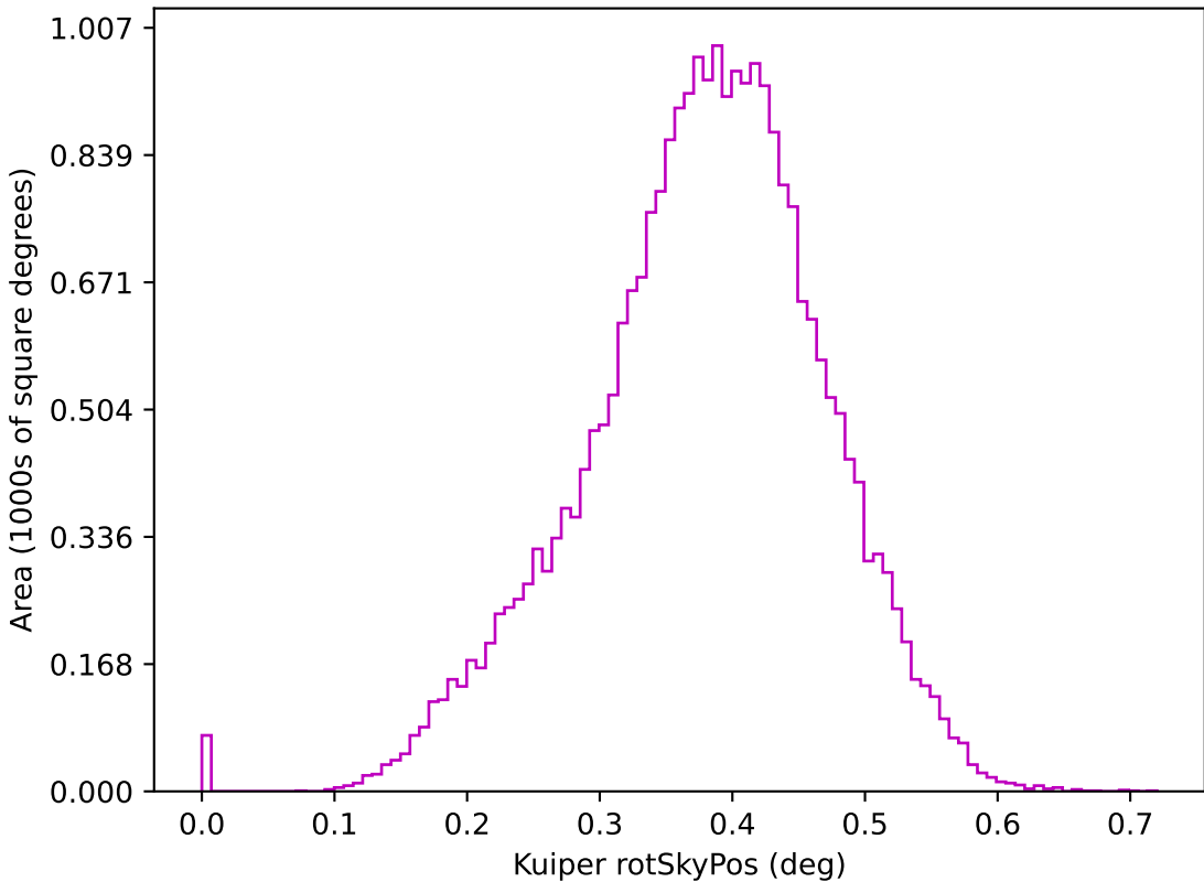
reweight_bulge_v3.3_10yrs z: Kuiper rotSkyPos
