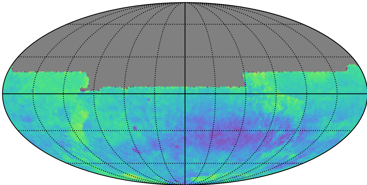
reweight_bulge_v3.3_10yrs y: Kuiper rotSkyPos
