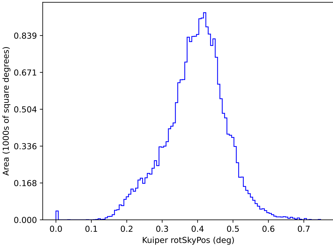
reweight_bulge_v3.3_10yrs y: Kuiper rotSkyPos
