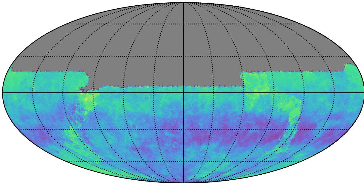
reweight_bulge_v3.3_10yrs u: Kuiper rotSkyPos
