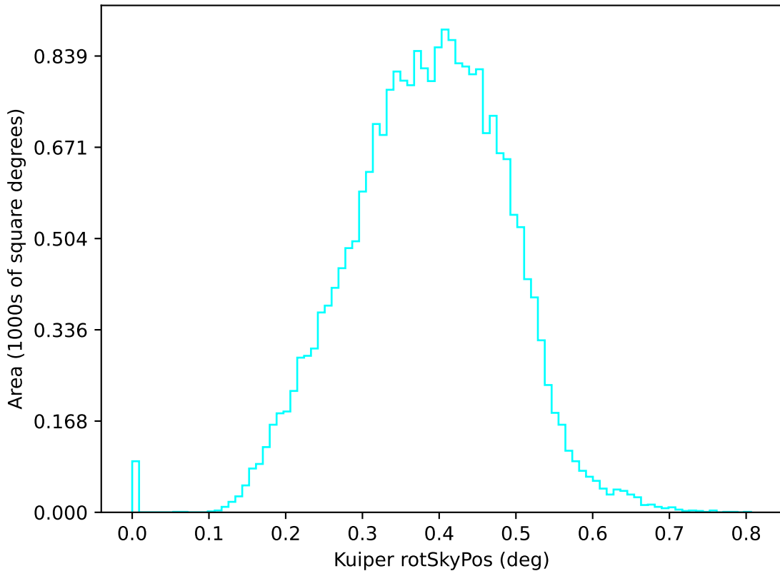
reweight_bulge_v3.3_10yrs u: Kuiper rotSkyPos
