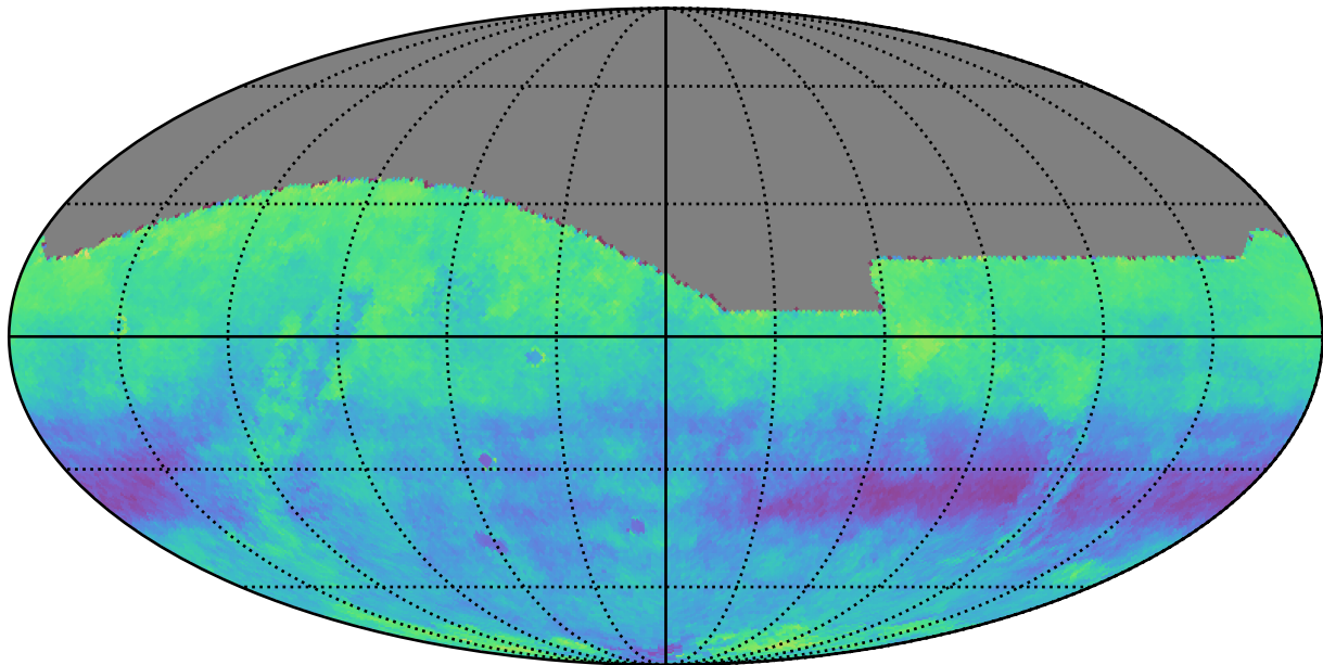
reweight_bulge_v3.3_10yrs r: Kuiper rotSkyPos
