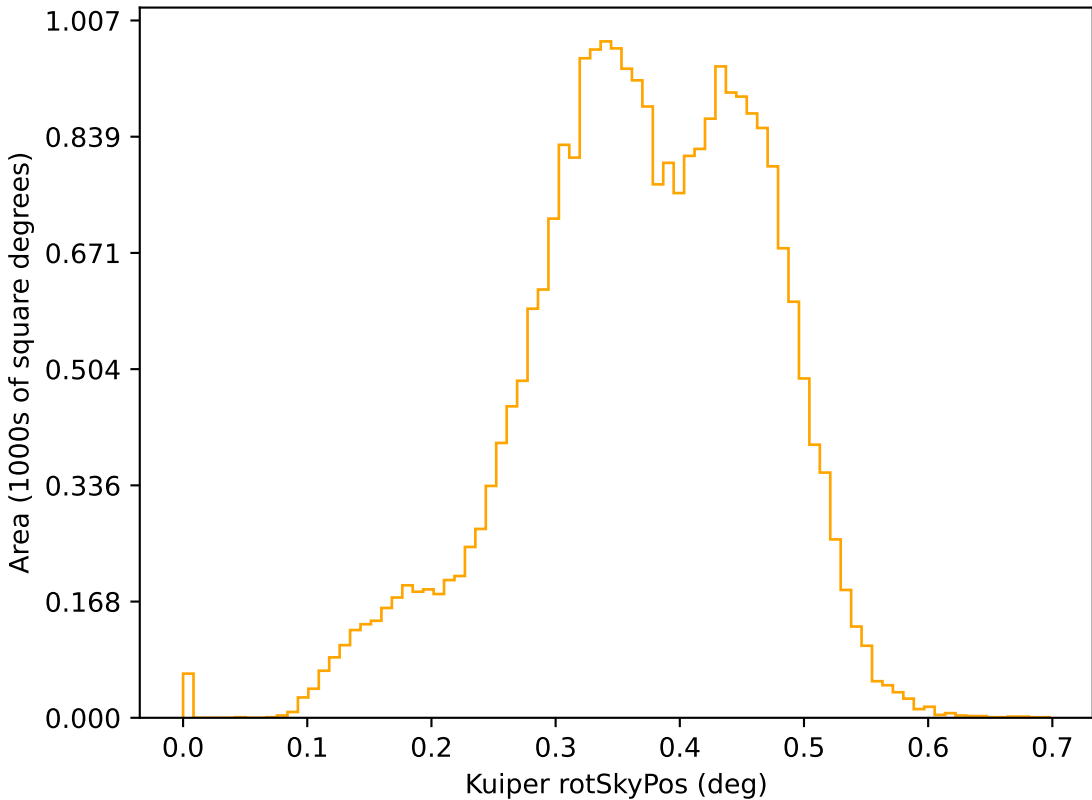
reweight_bulge_v3.3_10yrs r: Kuiper rotSkyPos
