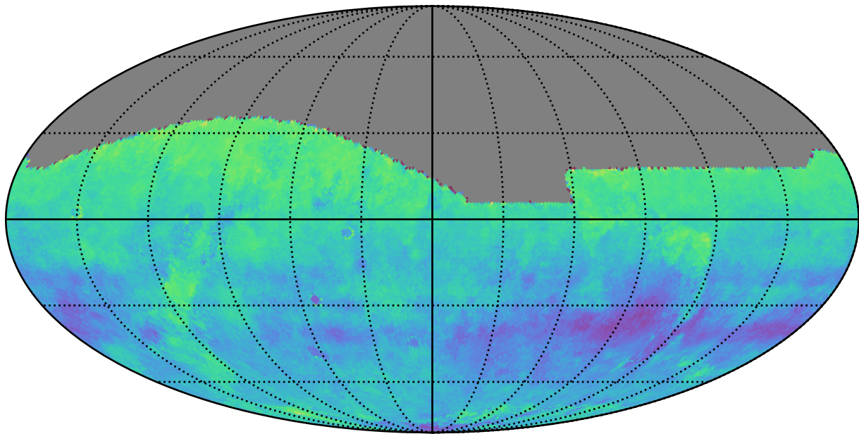
reweight_bulge_v3.3_10yrs i: Kuiper rotSkyPos
