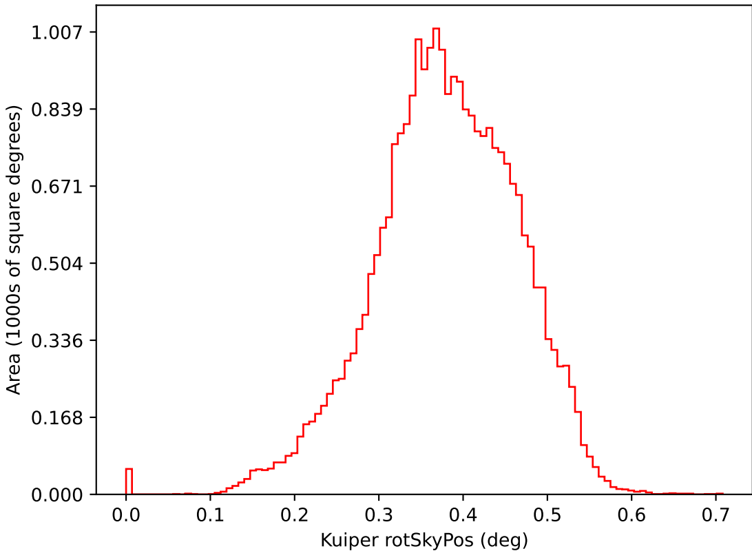
reweight_bulge_v3.3_10yrs i: Kuiper rotSkyPos
