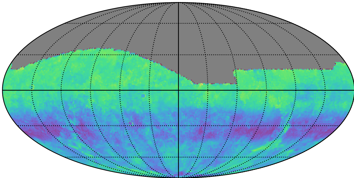
reweight_bulge_v3.3_10yrs g: Kuiper rotSkyPos
