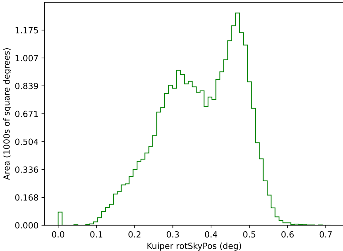
reweight_bulge_v3.3_10yrs g: Kuiper rotSkyPos
