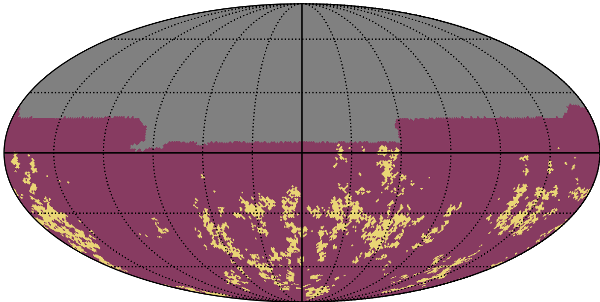
reweight_bulge_v3.3_10yrs u band: Gaps_7hr
