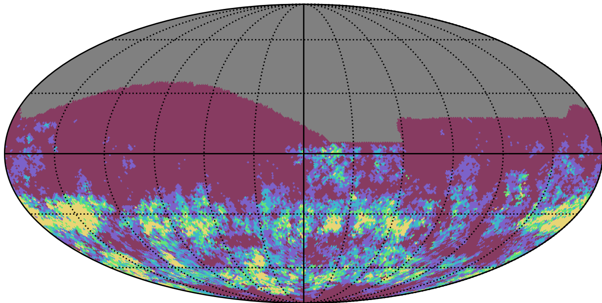
reweight_bulge_v3.3_10yrs r band: Gaps_7hr
