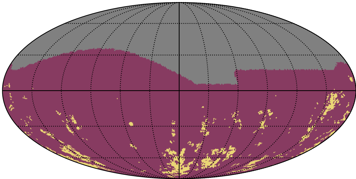
reweight_bulge_v3.3_10yrs g band: Gaps_7hr
