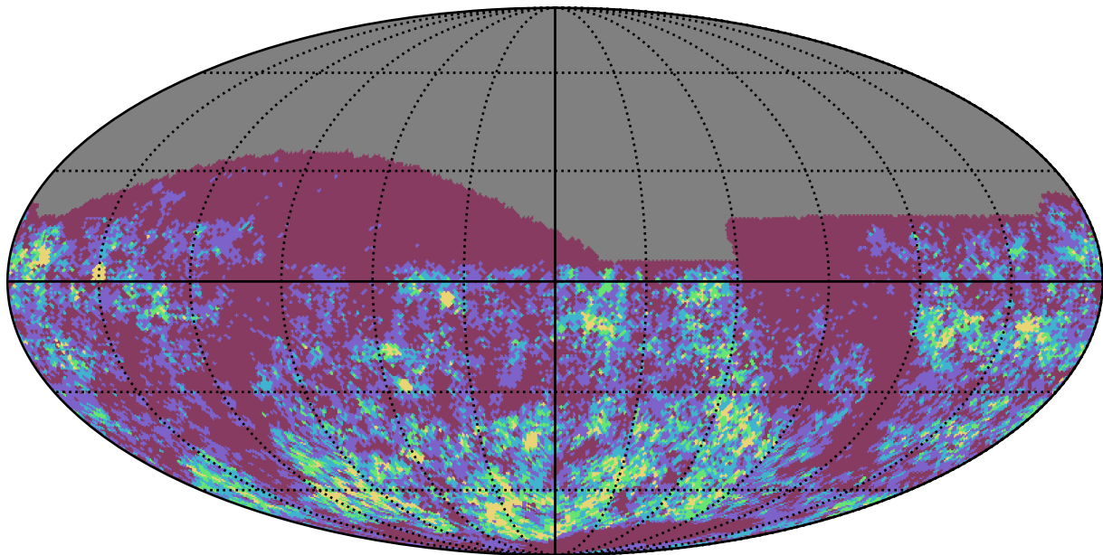
reweight_bulge_v3.3_10yrs z band: Gaps_3hr
