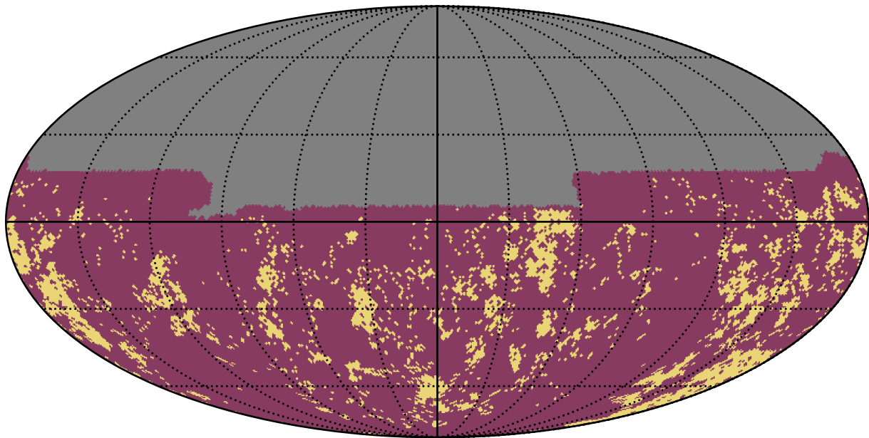
reweight_bulge_v3.3_10yrs u band: Gaps_3hr
