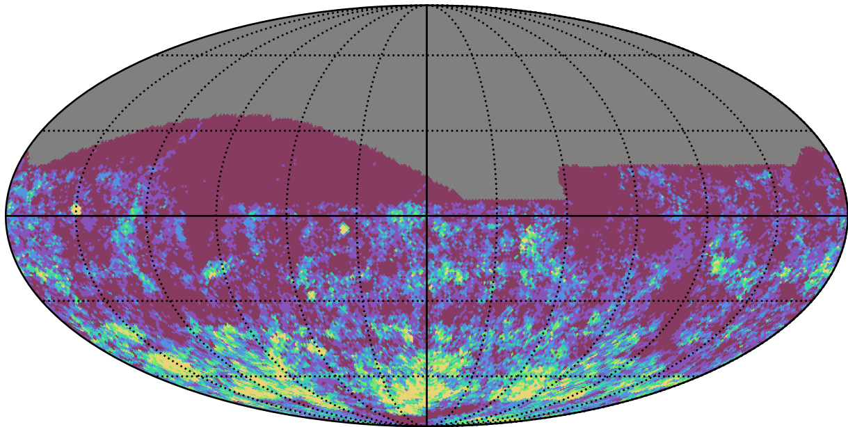
reweight_bulge_v3.3_10yrs r band: Gaps_3hr
