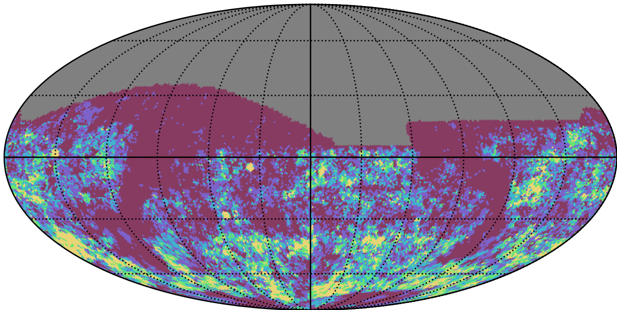
reweight_bulge_v3.3_10yrs i band: Gaps_3hr
