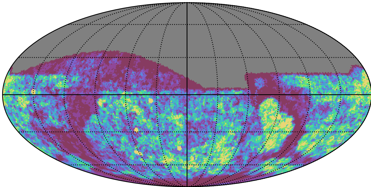
reweight_bulge_v3.3_10yrs g band: Gaps_24hr
