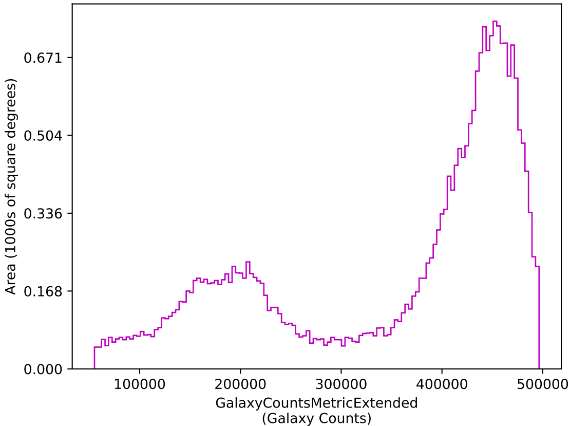
reweight_bulge_v3.3_10yrs z: GalaxyCountsMetricExtended
