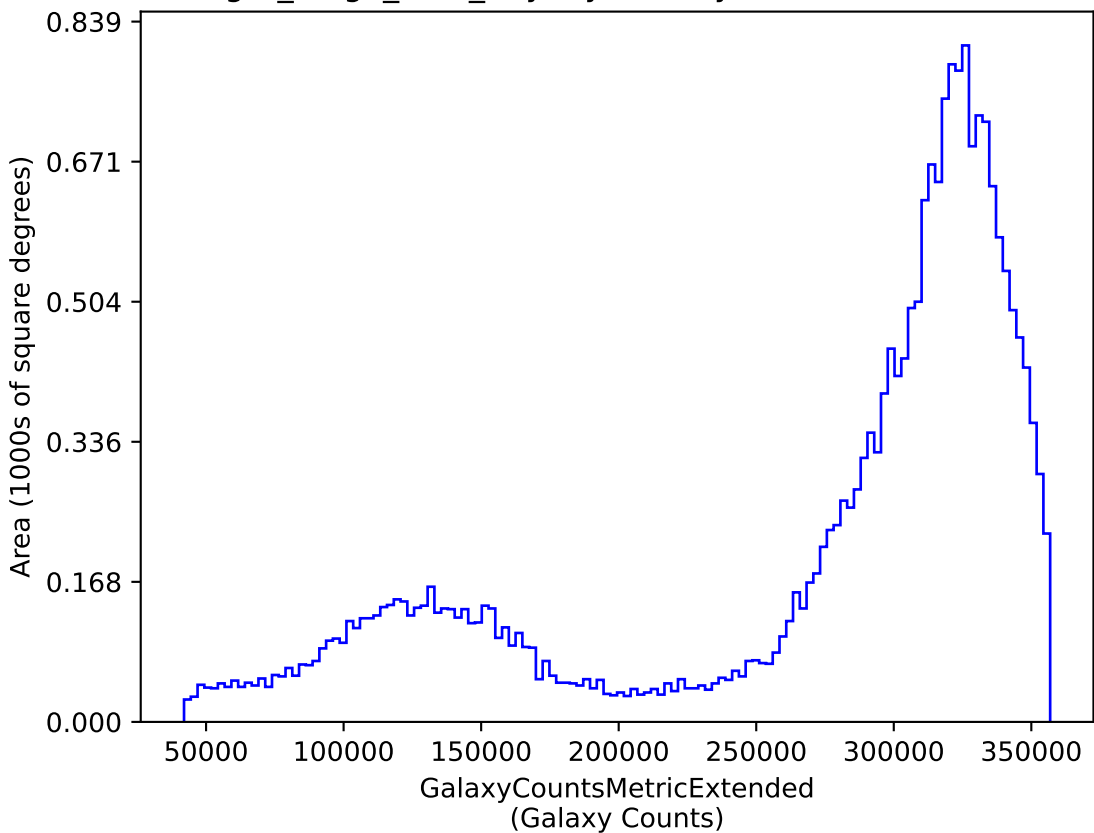
reweight_bulge_v3.3_10yrs y: GalaxyCountsMetricExtended
