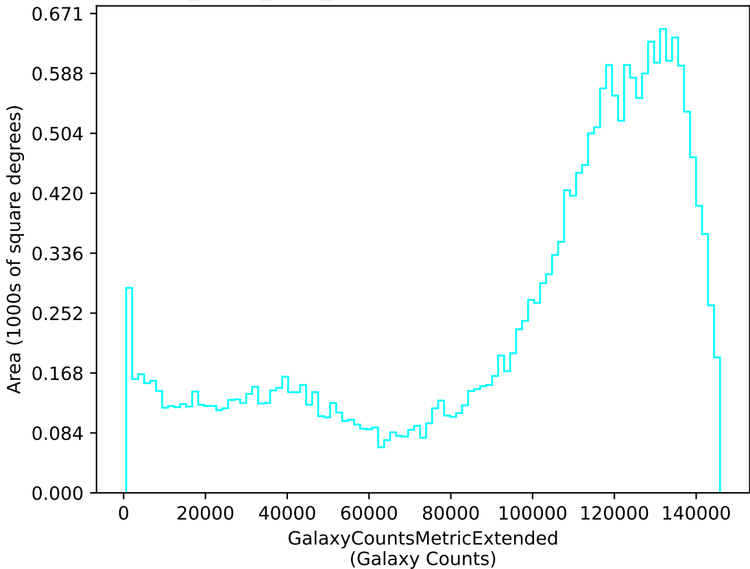
reweight_bulge_v3.3_10yrs u: GalaxyCountsMetricExtended
