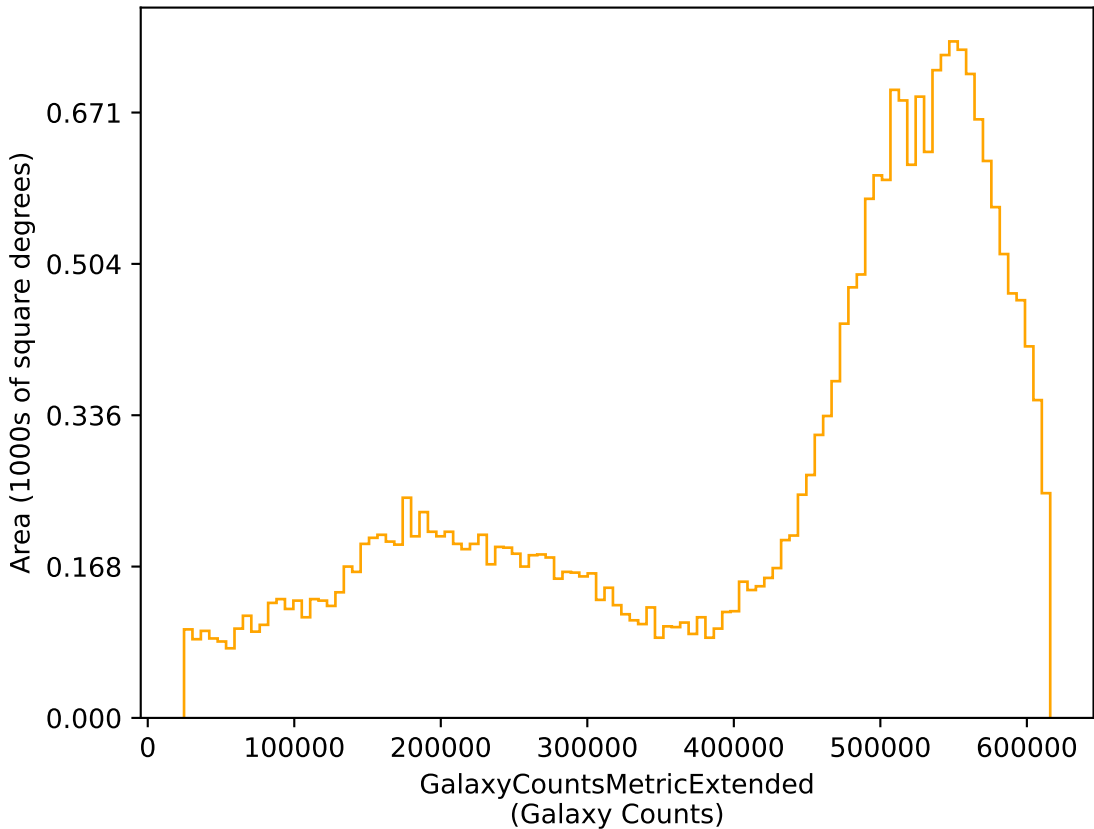
reweight_bulge_v3.3_10yrs r: GalaxyCountsMetricExtended
